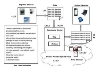
Figure 3: Classification of the top ten challenges Some other conveyed figuring issues in gigantic data:
