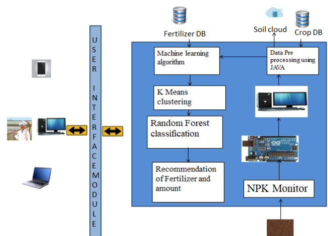
Figure1: Architectural diagram
