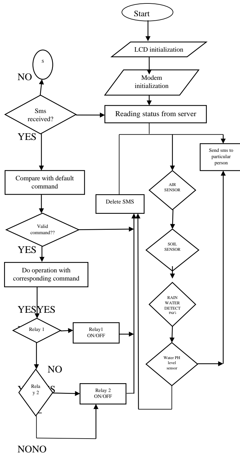
Fig 7 Flow Diagram of micro controller
