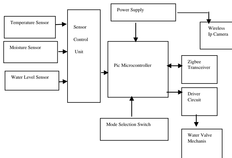
Fig 1 Sensor control unit
