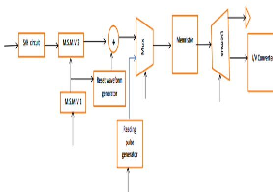
Figure 2. Basic Memory cell with S/H- Sample and Hold Circuit, MSMV-Multi State Multi Vibrator, I-Current, V-Voltage.
