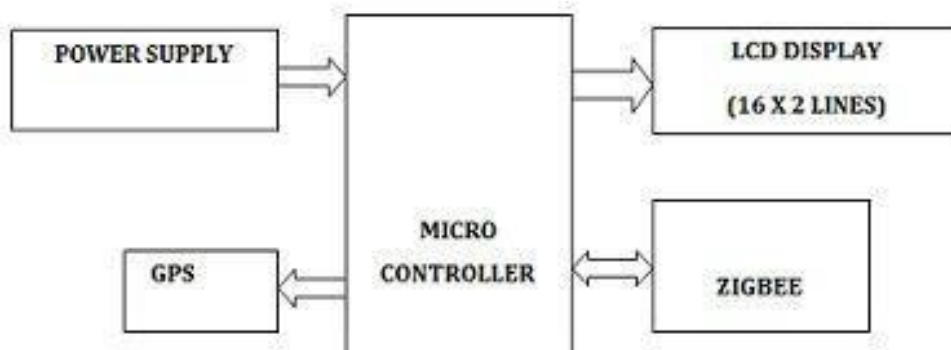
Fig 2: Bus unit.
