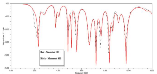
Fig 10: Comparison of measured & simulated S11
