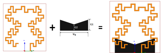
(a) MQKFA (b) DGS (c) MQKFDGA
