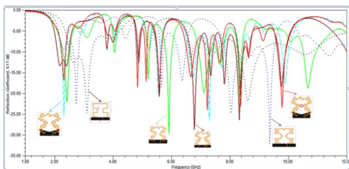
Fig 7: Return loss characteristics of various proposed antenna structures
