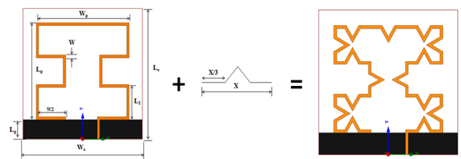
(a) Moore curve (b) Triangular Koch fractal (c) MTKFA
