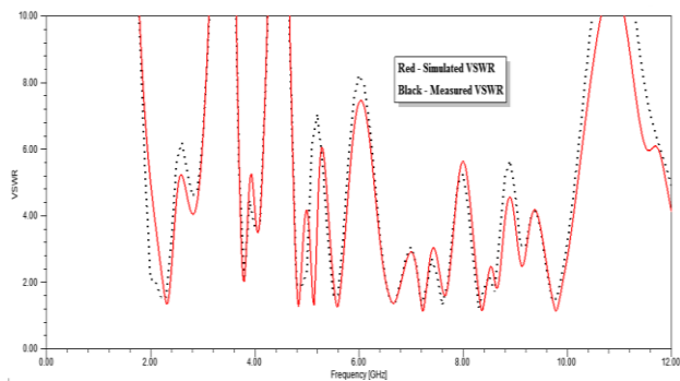
Fig 11: Comparison of measured & simulated VSWR
