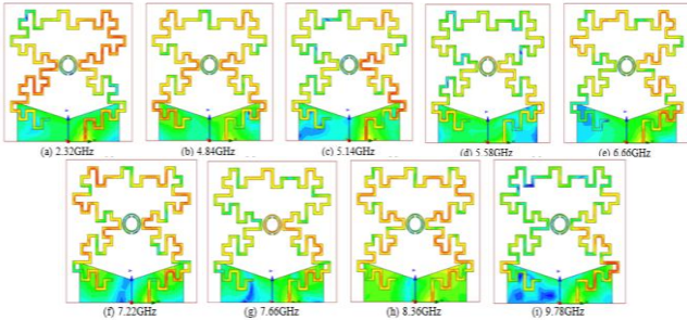
Fig 8: Magnitude surface current distribution of proposed antenna
