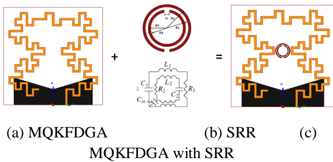
Fig 6: Design implementation of proposed MQKFDGA loaded with SRR
