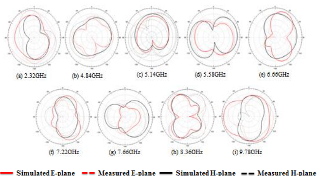
Fig 12: Radiation patterns of the proposed antenna
