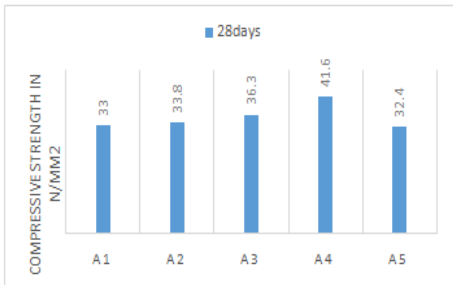
Fig.6.2: Compressive Strength test results (Acid Attack @ 60 DAYS)
