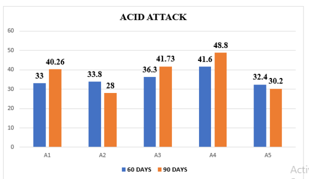
Compressive Strength test results (Acid Attack)
