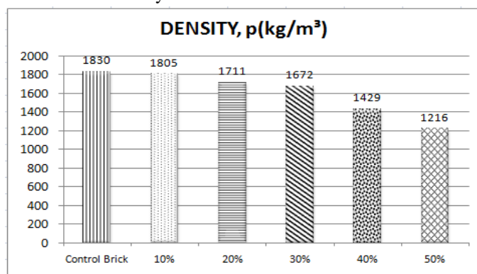
Figure 3: Density with different percentage of GB
