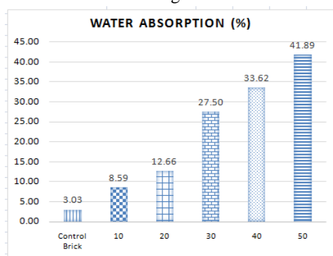
Figure 2: Water absorption with different percentages of GB
