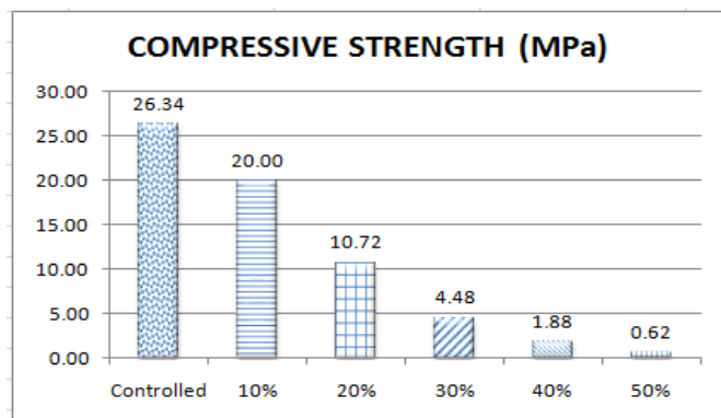
Figure 4: Compressive strength with different percentages of GB
