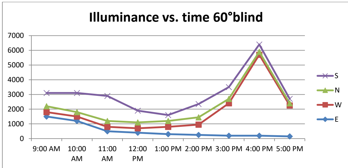
Fig.10. Illuminance vs. Time for 60° blinds
