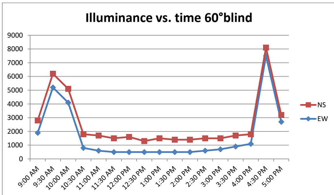
Fig.5. Illuminance vs. Time for 60° blinds
