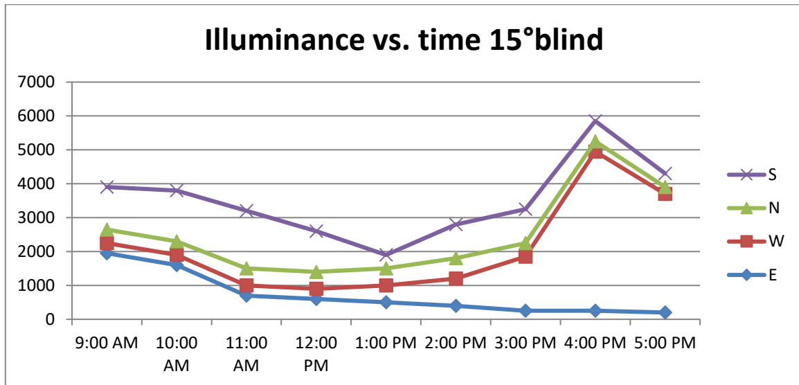
Fig.7. Illuminance vs. Time for 15° blinds
