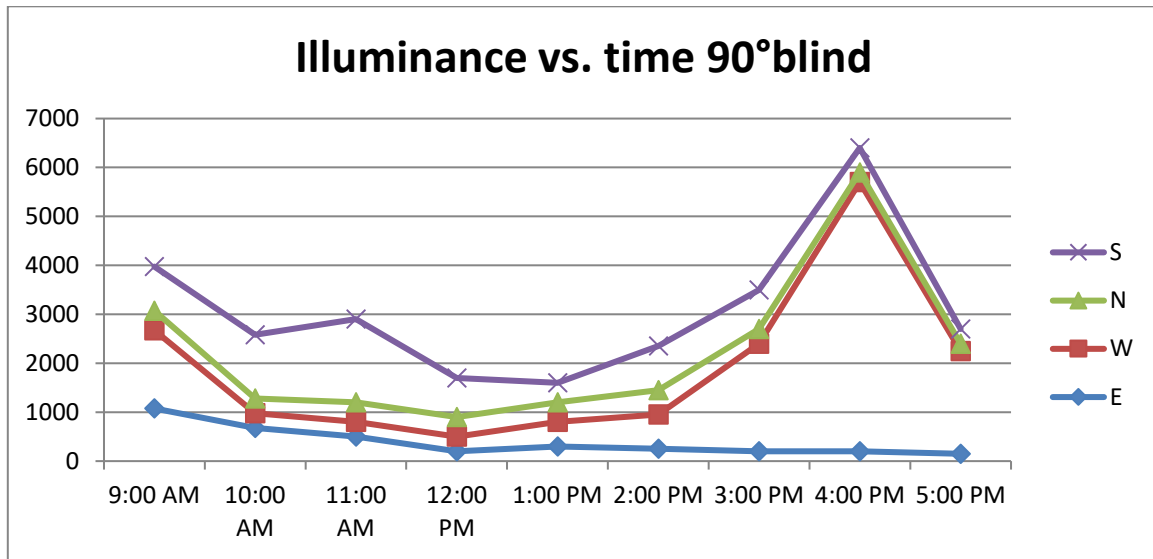
Fig.12. Illuminance vs. Time for 90° blinds
