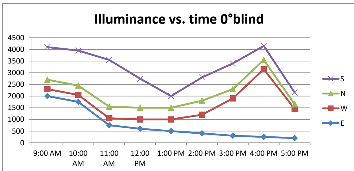
Fig.6. Illuminance vs. Time for 0° blinds
