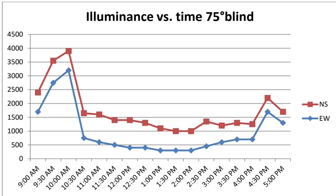
Fig.6. Illuminance vs. Time for 75° blinds
