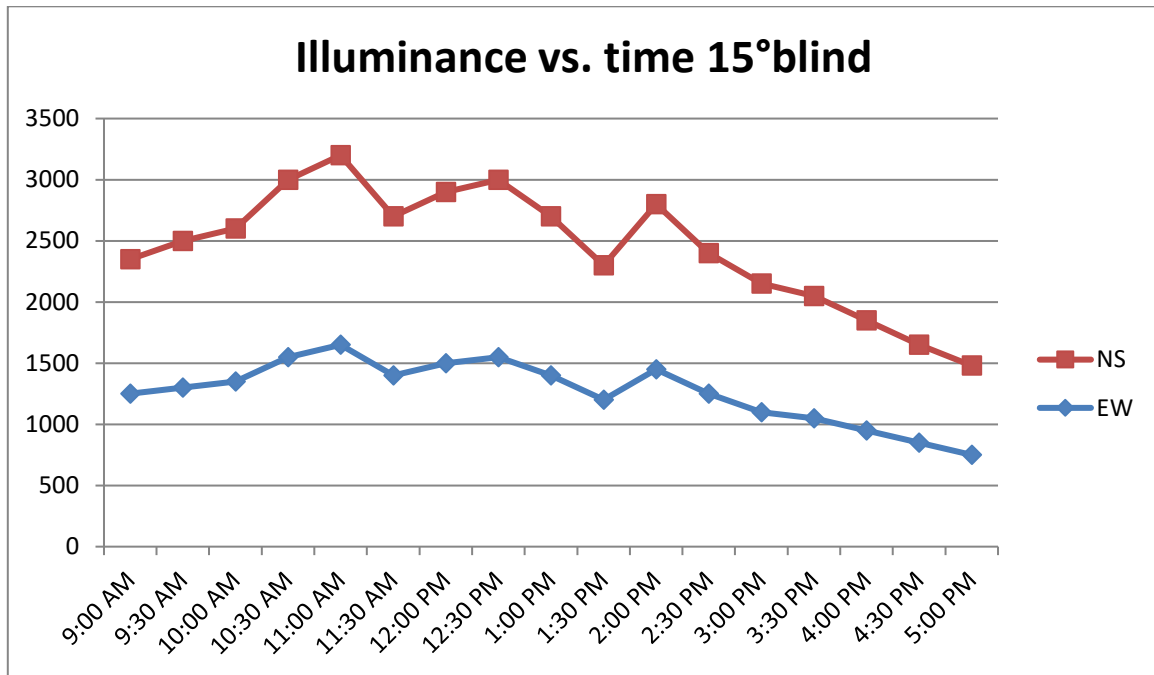
Fig.2. Illuminance vs. Time for 15° blinds
