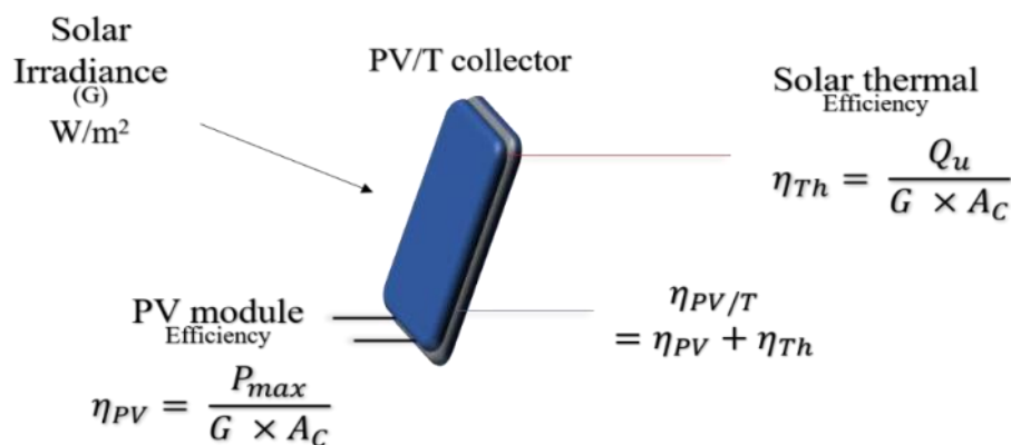
Fig. 3 Efficiency equations of PVT
